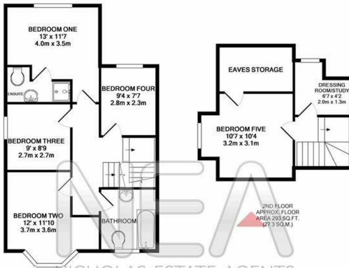
1ST FLOOR APPROX. FLOOR AREA 604 SQ.FT. (56.1 SQ.M.)
